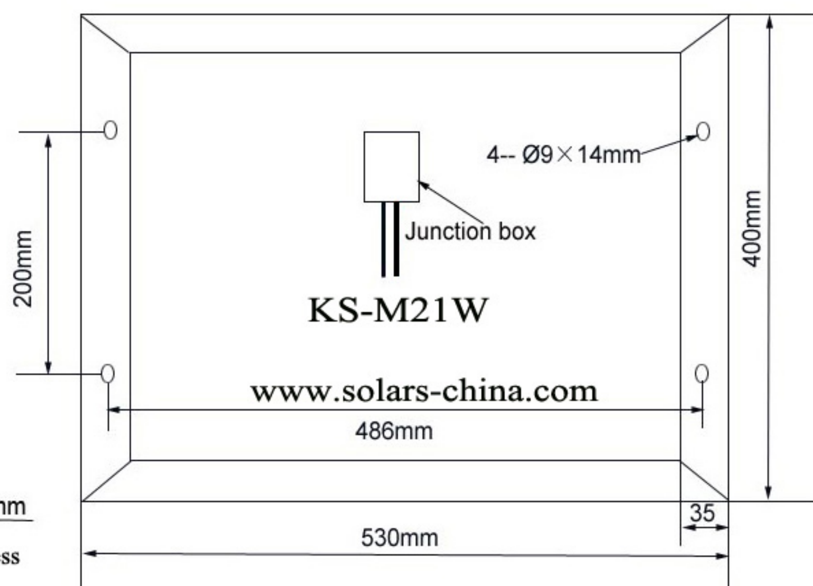
BACK VIEW
