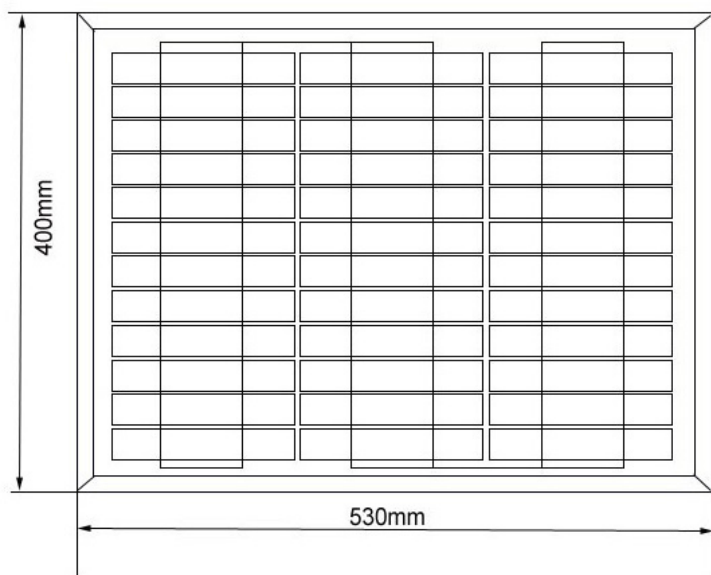
FRONT VIEW
