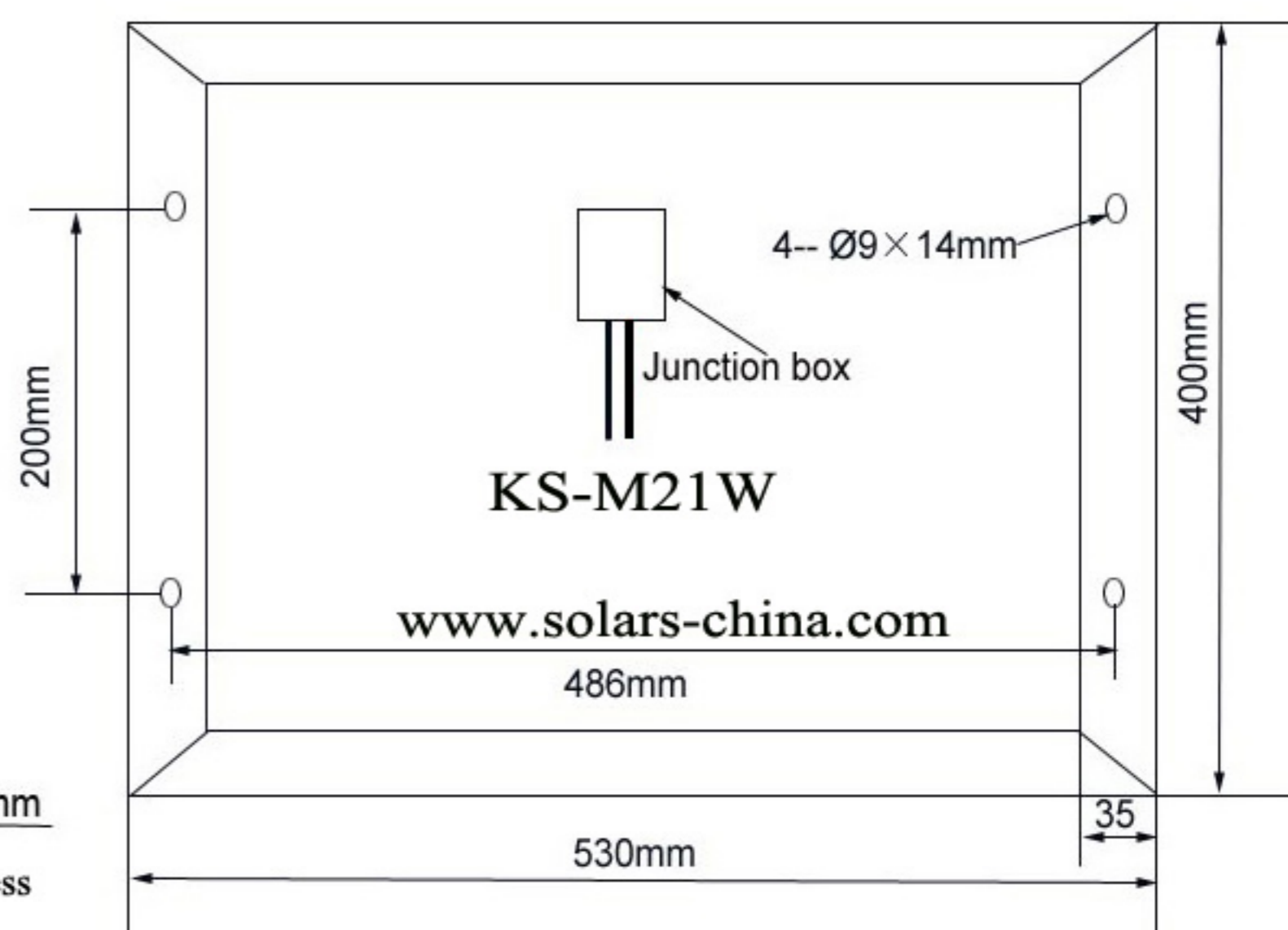
BACK VIEW
