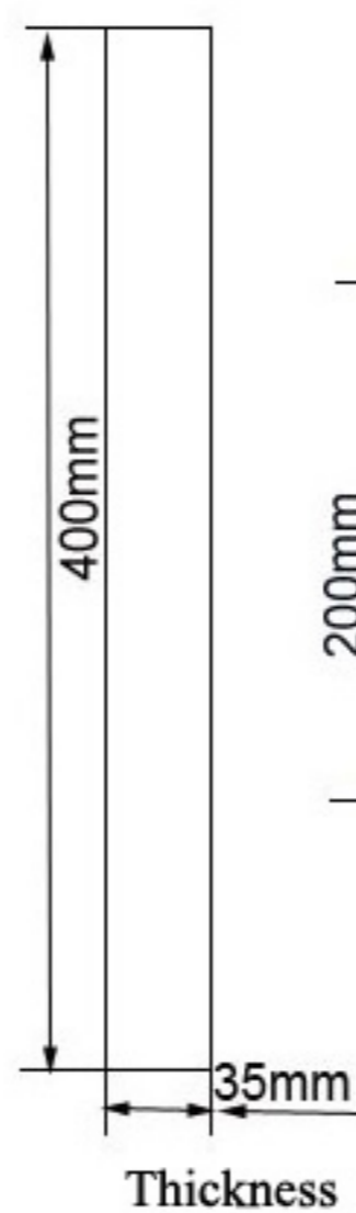
SIDE VIEW
