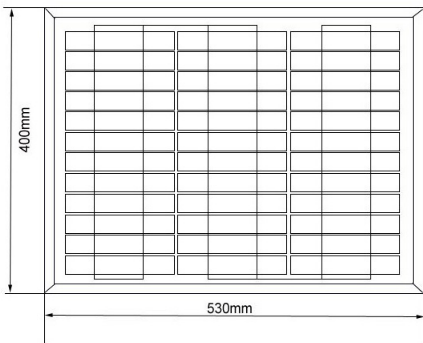
FRONT VIEW
