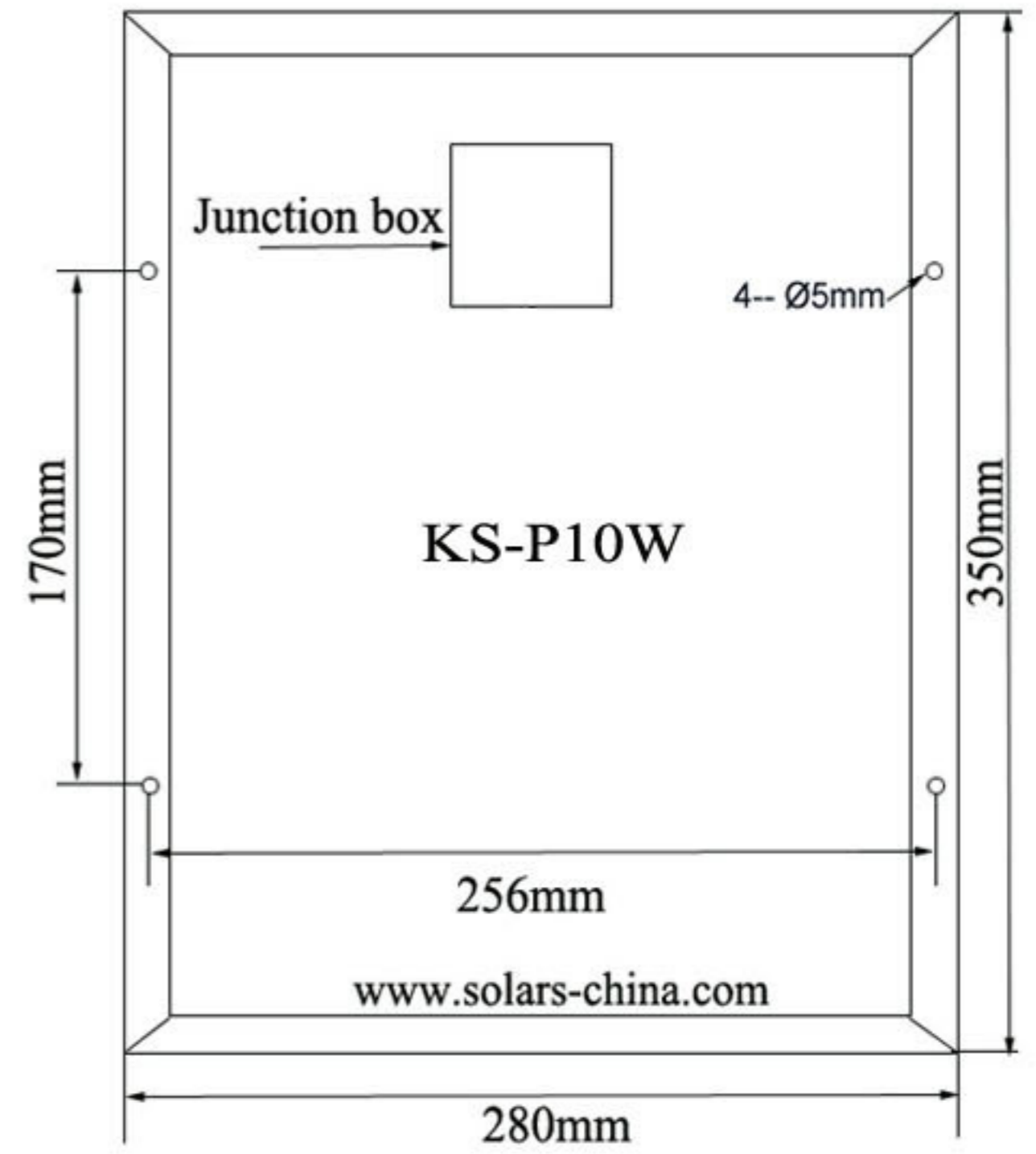
BACK VIEW
